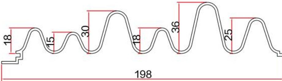
Assembly drawing
